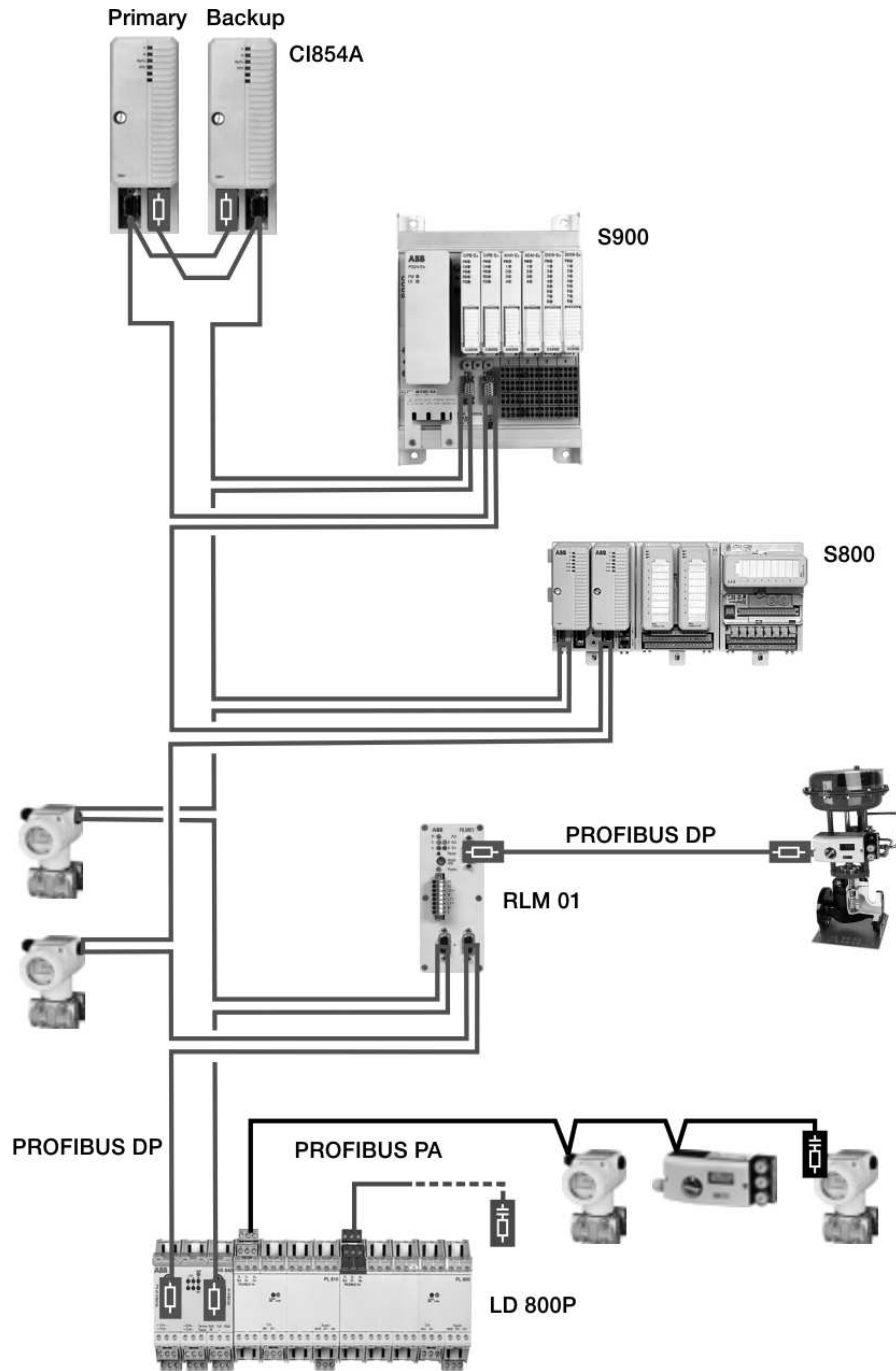
Figure 34. Master, Line and Slave Redundancy
