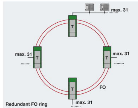
Redundant FO ring
